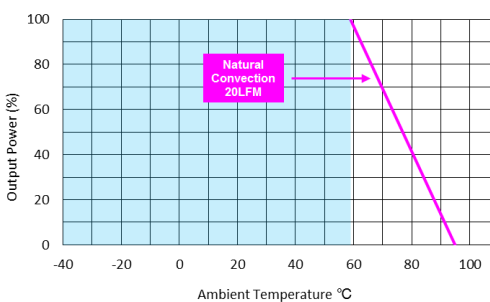
MKE15-12S05HI, MKE15-12S051HI
