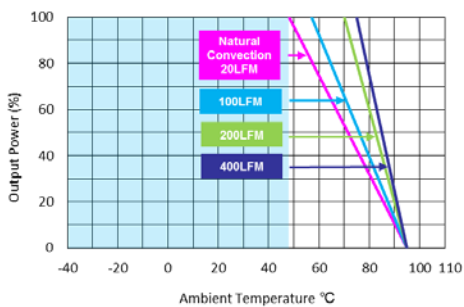
MKE20-12S05HI, MKE20-12S051HI
