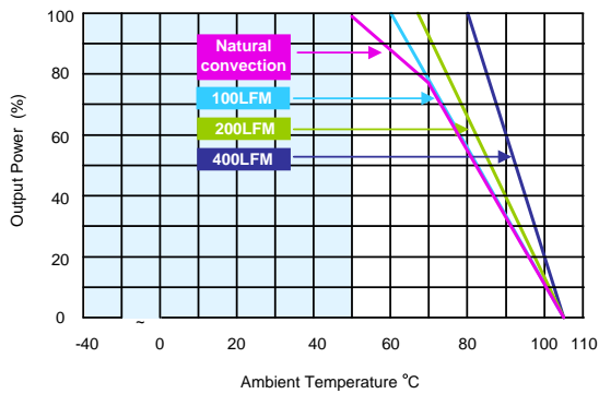
Derating Curve without Heatsink
