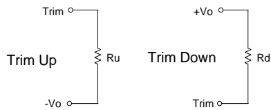
MKZI20-XXS05 Trim Table
