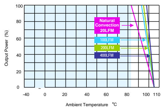
MKZ110-110S05 Derating Curve with Heatsink
