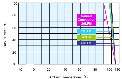
MKZI10-24S15, MKZI10-24D15, MKZI10-48S12, MKZI10-48S15 Derating Curve with Heatsink
