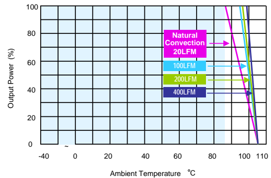
MKZ110-24S05 Derating Curve with Heatsink
