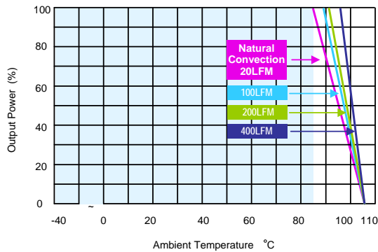
MKZ110-48S05, MKZ110-110S12, MKZ110-110S15, MKZ110-110S24 Derating Curve without Heatsink
