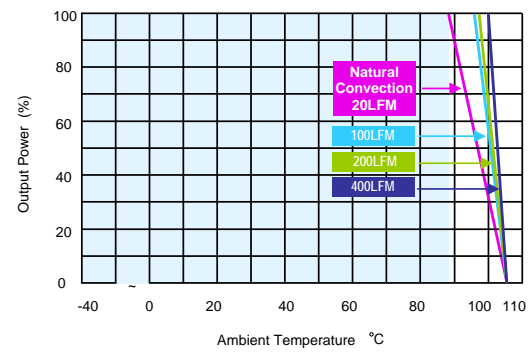
MKZ110-48S05, MKZ110-110S12, MKZ110-110S15, MKZ110-110S24 Derating Curve with Heatsink
