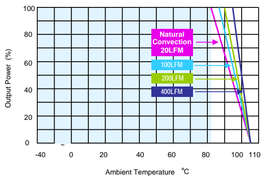
MKZ110-24S05 Derating Curve without Heatsink
