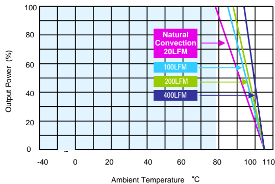
MKZ110-110S05 Derating Curve without Heatsink
