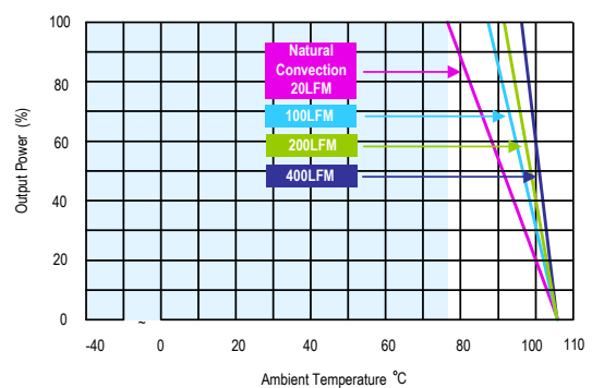
MJWI15-24S15, MJWI15-24D12, MJWI15-24D15, MJWI15-48S12, MJWI15-48S15, MJWI15-48D15 Derating Curve with Heatsink
