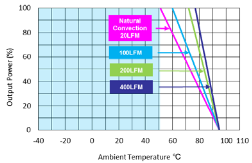
MKW20-12S05M, MKW20-12S051M
