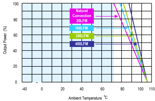
MJWI15-24S033, MJWI15-48S033 Derating Curve without Heatsink
