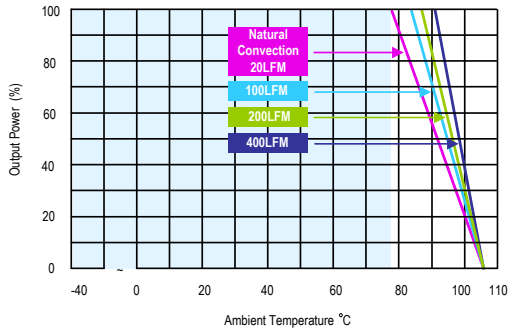
MJWI15-24S24, MJWI15-48S24 Derating Curve without Heatsink
