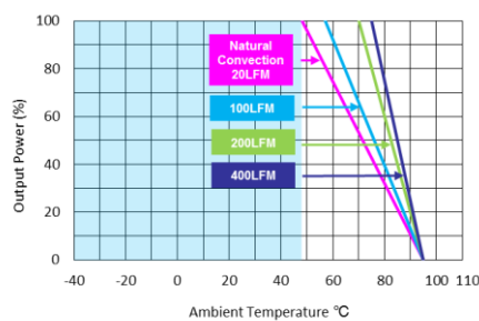
MKE20-12S05HI, MKE20-12S051HI
