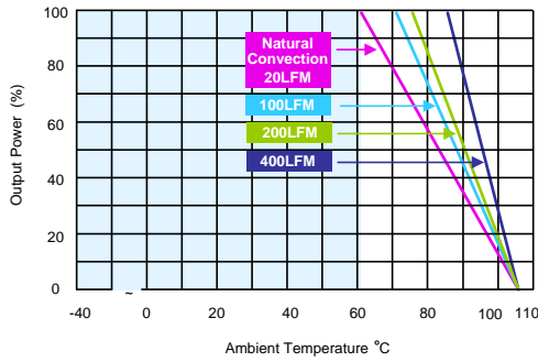
MKW150-24S033, MKW150-48S033 Derating Curve without Heatsink
