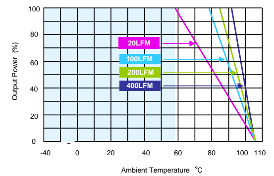
MJW25-12S05, MJW25-12S12, MJW25-12S15, MJW25-12D12 MJW25-12D15, MJW25-24D12, MJW25-24D15, MJW25-48D12, MJW25-48D15 Derating Curve with Heatsink
