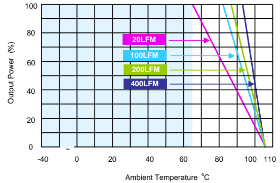
MJW25-24S033, MJW25-48S033 Derating Curve with Heatsink
