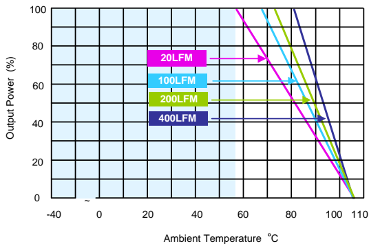
MJW25-24S033, MJW25-48S033 Derating Curve without Heatsink
