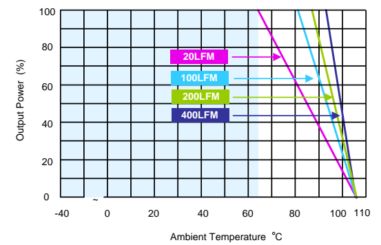
MJW25-24S05, MJW25-24S12, MJW25-24S15, MJW25-48S05 MJW25-48S12, MJW25-48S15 Derating Curve with Heatsink
