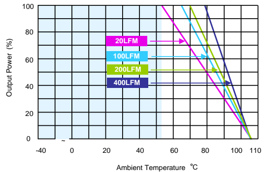
MJW25-12S033 Derating Curve without Heatsink
