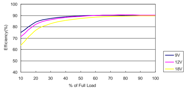
MJW25-12D15 Efficiency vs Load Current
