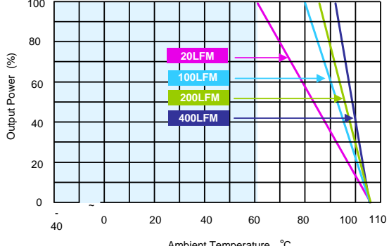
MJW25-12S033 Derating Curve with Heatsink
