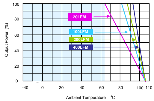
MJWI25-24S15, MJWI25-48S05, MJWI25-48S12, MJWI25-48S15 Derating Curve with Heatsink
