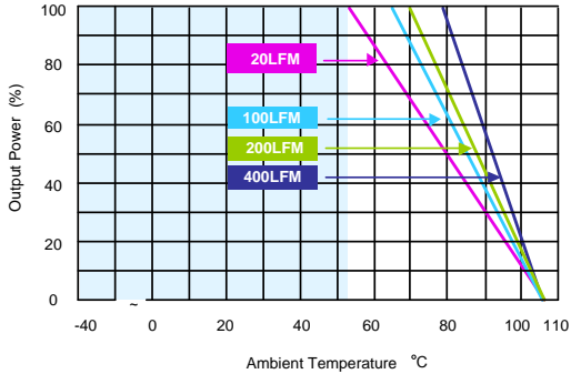
MJWI25-24S033 Derating Curve without Heatsink
