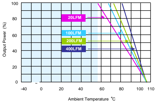
MJWI25-48S033 Derating Curve without Heatsink
