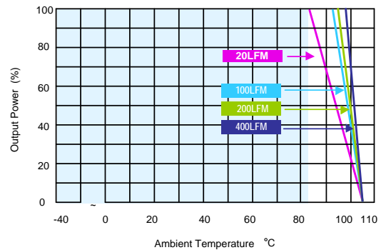
MKZ110-110S05 Derating Curve with Heatsink
