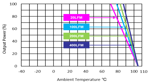
MJW15-12S05, MJW15-12S12, MJW15-12S15, MJW15-12D12 MJW15-48D12 Derating Curve without Heatsink
